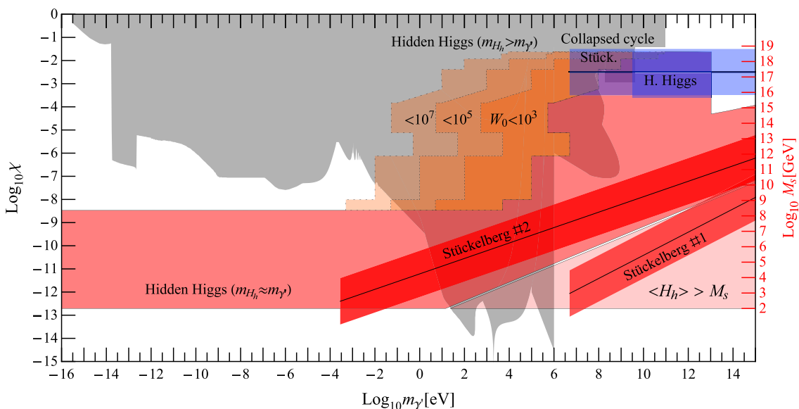
Figure 11. String theory expectations for the mass and kinetic mixings of massive hidden U(1) gauge bosons kinetically mixing with the ordinary electromagnetic photon. The red/orange areas denote a situation where the hidden U(1) arises from a hyperweak D7 brane. In this case the kinetic mixing is directly related (up to an order of magnitude) to the string scale M_s , which is shown on the right axis. The straight bands denote the situations where the hidden photon mass arises from a Stückelberg mechanism. The lighter red area extending to arbitrarily low masses shows the possible masses from a Higgs mechanism. The lower bound comes from a lower bound to the string scale M_s > 100 GeV. In the lower right triangle (lighter red) shows a region where the vacuum expectation value of the hidden Higgs would be larger than the string scale ( \langle H_h \rangle > M_s ). The upper bound on the kinetic mixing comes from constraints on the phenomenology of the hidden Higgs particle which becomes mini-charged (cf. section 5.1 and [28]). All the red areas correspond to the natural case where the hidden Higgs mass is similar to that of the hidden photon ( m_{H_h} \approx m_{\gamma'} \approx m_{\text{soft}}^{\text{hid}} ). However, in models with a chiral Higgs it is possible to create a hierarchy ( m_{H_h} \gg m_{\gamma'} ) by tuning W_0 , which make the regions shown in orange phenomenologically allowed. The blue bands correspond to the case where the hidden photon arises from a collapsed cycle and either gains its mass through a Stückelberg or a hidden Higgs mechanism. For comparison we have included the current experimental constraints as the grey area (cf. figure 1 for details).
