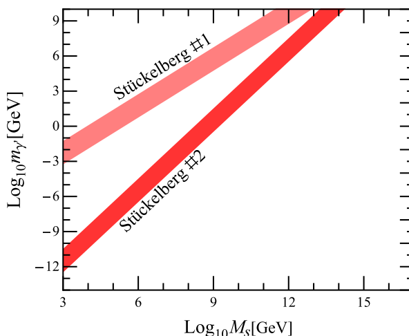
Figure 7. Stueckelberg mass term of the hidden U(1) on a hyperweak, bulk D7 brane wrapping a 4-cycle from the estimates in (4.9) (#1, light red) and (4.10) (#2, dark red).
