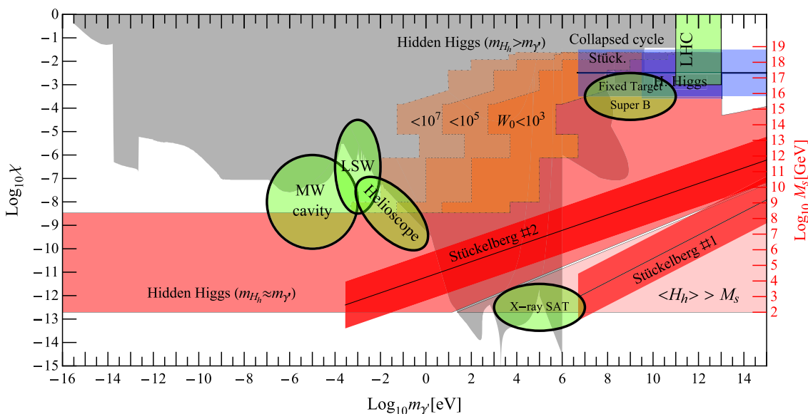
Figure 12. As in figure 11 but in addition we show some interesting future probes of massive hidden U(1)s like: light-shining-through-a-wall (LSW) experiments with optical lasers [18] or with microwaves in resonant cavities [21, 24–27], helioscopes looking for hidden photons emitted from the Sun [22, 124, 125], the extragalactic X-ray diffuse background [31], e^+e^- colliders [37, 45], fixed-target experiments [38, 46], and hadron colliders like Tevatron or the LHC [35, 36].
