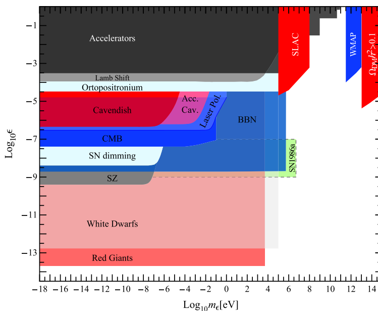
Figure 8. Constraints on the existence of minicharged particles with electrical charge (in units of the elementary electric charge e ) \epsilon and mass m_\epsilon [14, 102–111]. The bounds are usually quoted for models without hidden photons, but the most relevant are also valid where the minicharge arises from kinetic mixing and the hidden photon mass is smaller or comparable to m_\epsilon (The WMAP bound of [111] is an exception.).
